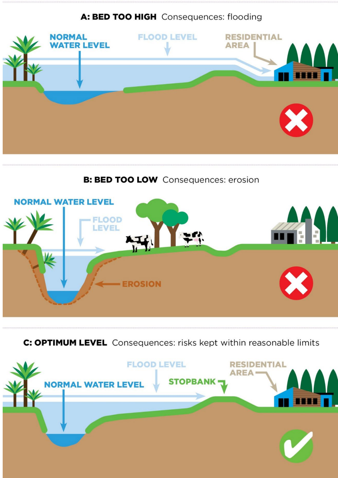
Figure 4 Gravel extraction strategy – optimum bed levels.
