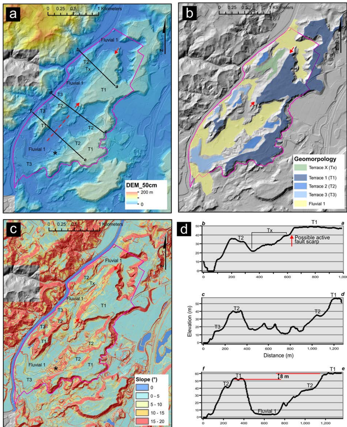
Figure 2.2 (a) Digital elevation and hillshade LiDAR DEM of the Tauriko West area. The location of the topographic lineation is shown by the red arrows. Red dashed line shows the along-strike projection of the lineation, * shows the location of landslide debris at the base of terrace risers and the black lines show the locations of the topographic profiles of figure (d). (b) Geomorphic map of the terrace surfaces (both volcanic and fluvial) in the area. (c) Slope DEM of the Tauriko West area. The river terrace risers, which are typically irregular and steep (15 – 20°) are shown well by this imagery. (d) Topographic profiles from across the possible active fault scarp and its along-strike projection. We show the possible faulted offset of surface T1 in profile e-f.
