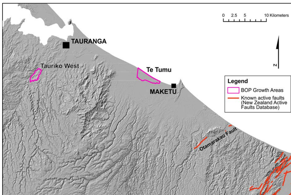
Figure 1.1 The Tauriko West and Te Tumu growth areas in the Bay of Plenty, shown on a hillshade LiDAR digital elevation model with the location of previously identified nearby active faults (Langridge et al. 2016).
