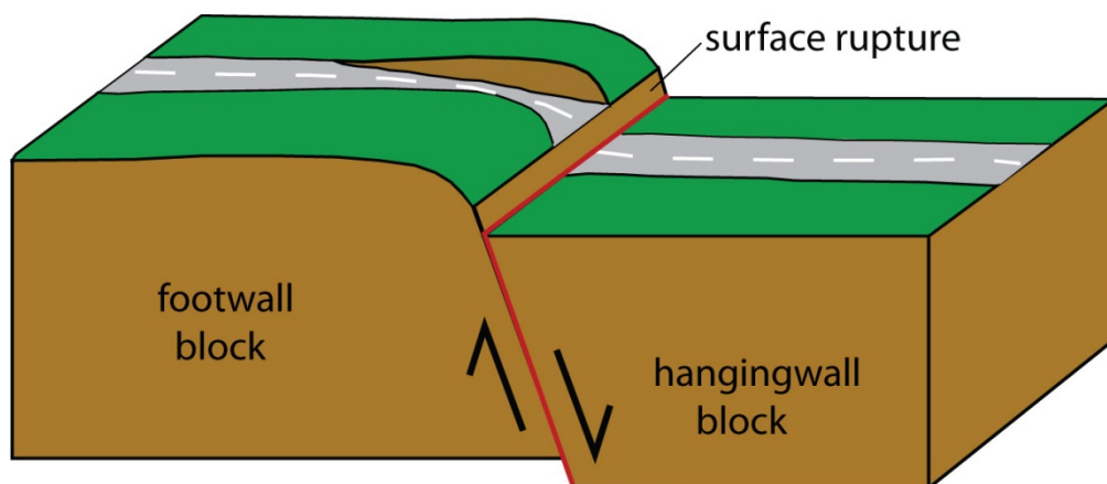
Figure A1.1 Block model of a normal dip-slip fault, typical of the TVZ faults. The relative movement of the blocks is vertical and in the dip direction of the fault plane. The hanging-wall block has dropped down, enhancing the height of the fault scarp.
