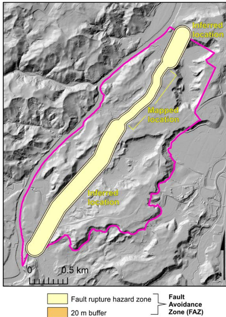
Figure 2.3 The FAZ for the possible active fault scarp in the Tauriko West area. Note that we can only map the possible fault scarp location across the higher T1 terrace; we infer the fault location across the low elevation floodplain and in this area there is a much higher locational uncertainty as the possible fault is concealed, resulting in a wider FAZ.
