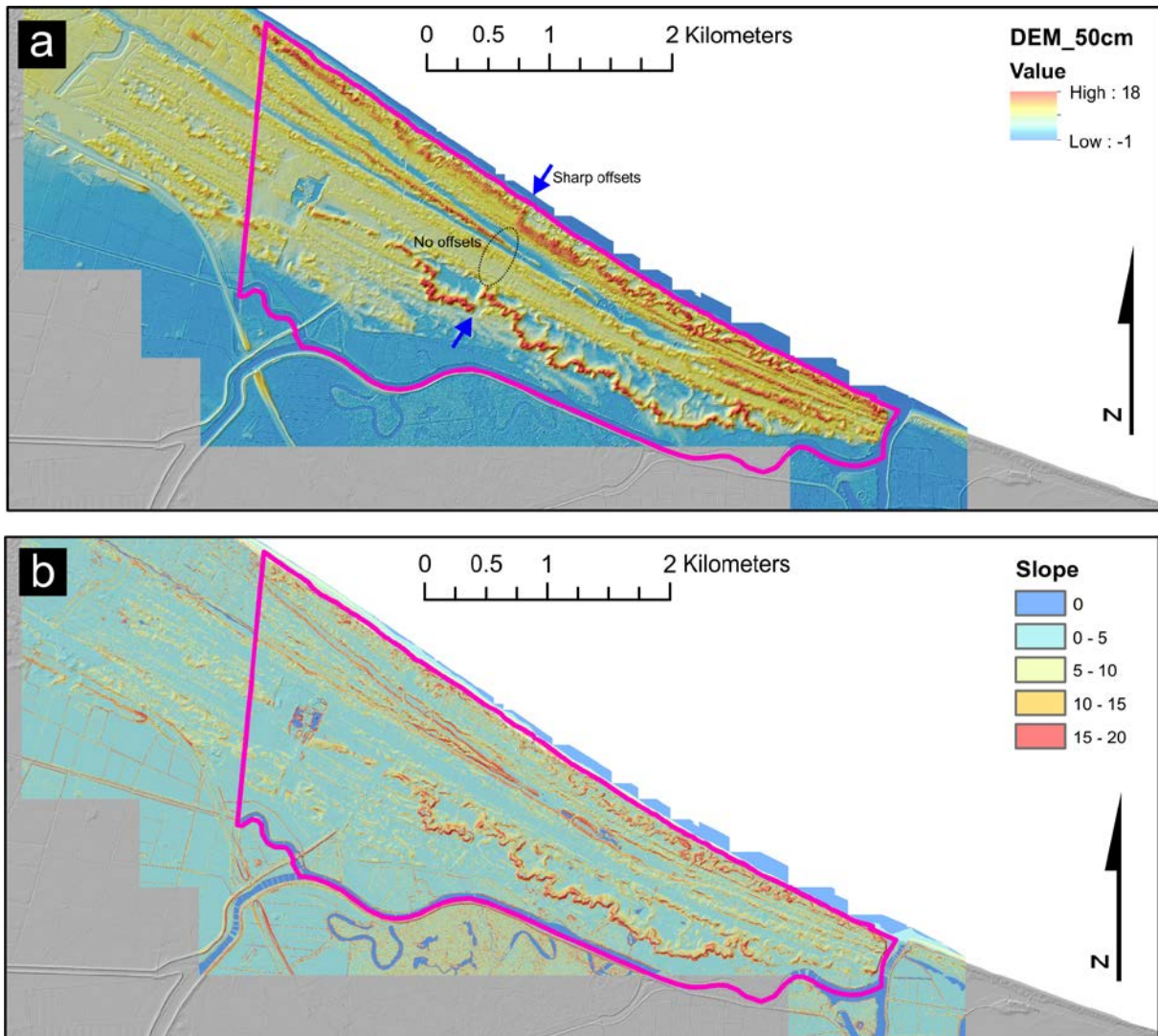
Figure 3.2 (a) Digital elevation and hillshade topographic LiDAR DEM of the Te Tumu area. The location of a lineation is shown by the blue arrows. (b) Slope DEM of the Te Tumu area. No scarp features compatible with active faults are seen.
