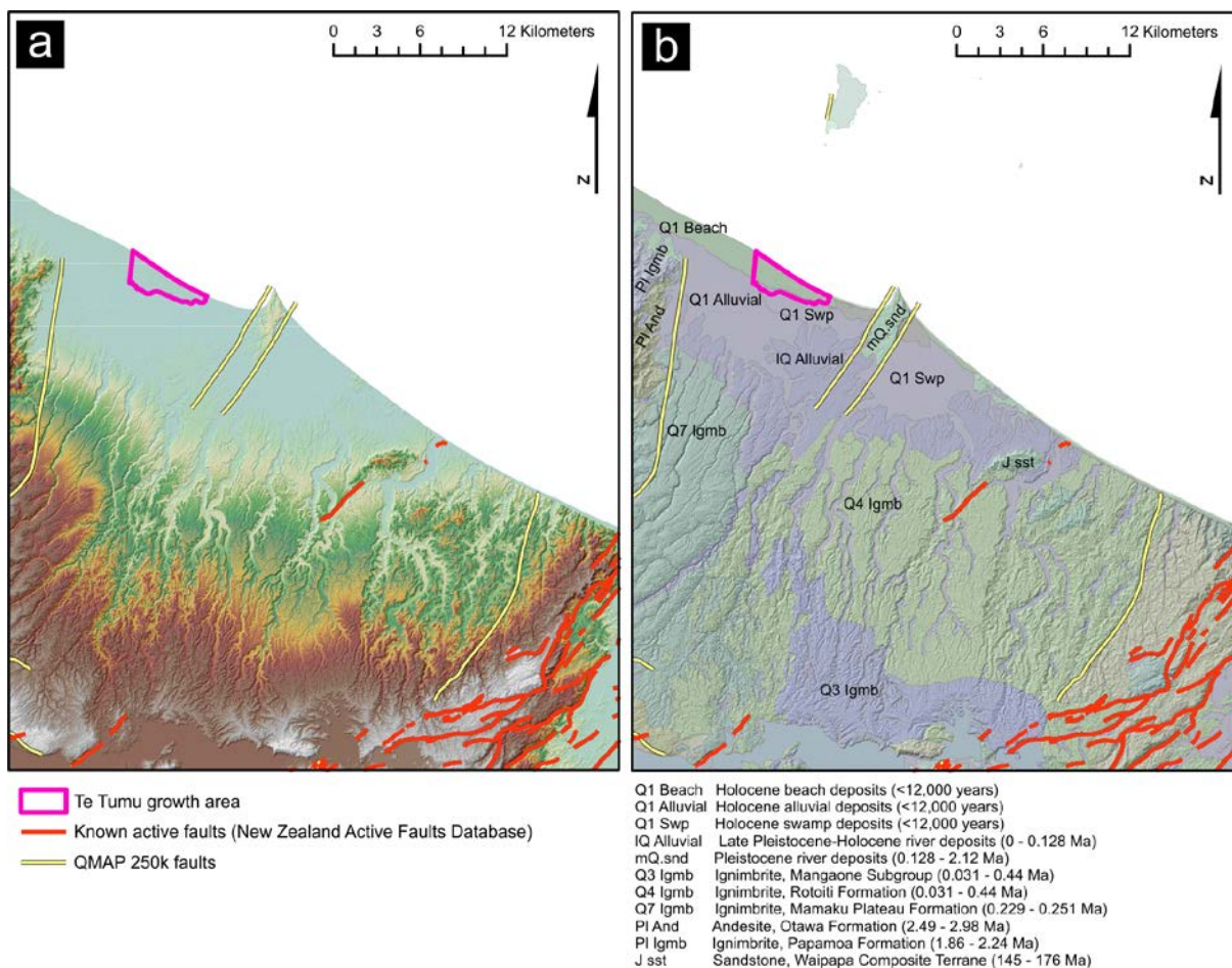
Figure 3.1 (a) A digital elevation and hillshade LiDAR DEM of the topography of the region surrounding Te Tumu. Onshore active faults from the NZ Active Faults database (Langridge et al. 2016), inactive faults from Leonard et al. (2010). (b) The geology and surface ages of the Te Tumu area, geological mapping from Leonard et al. (2010).
