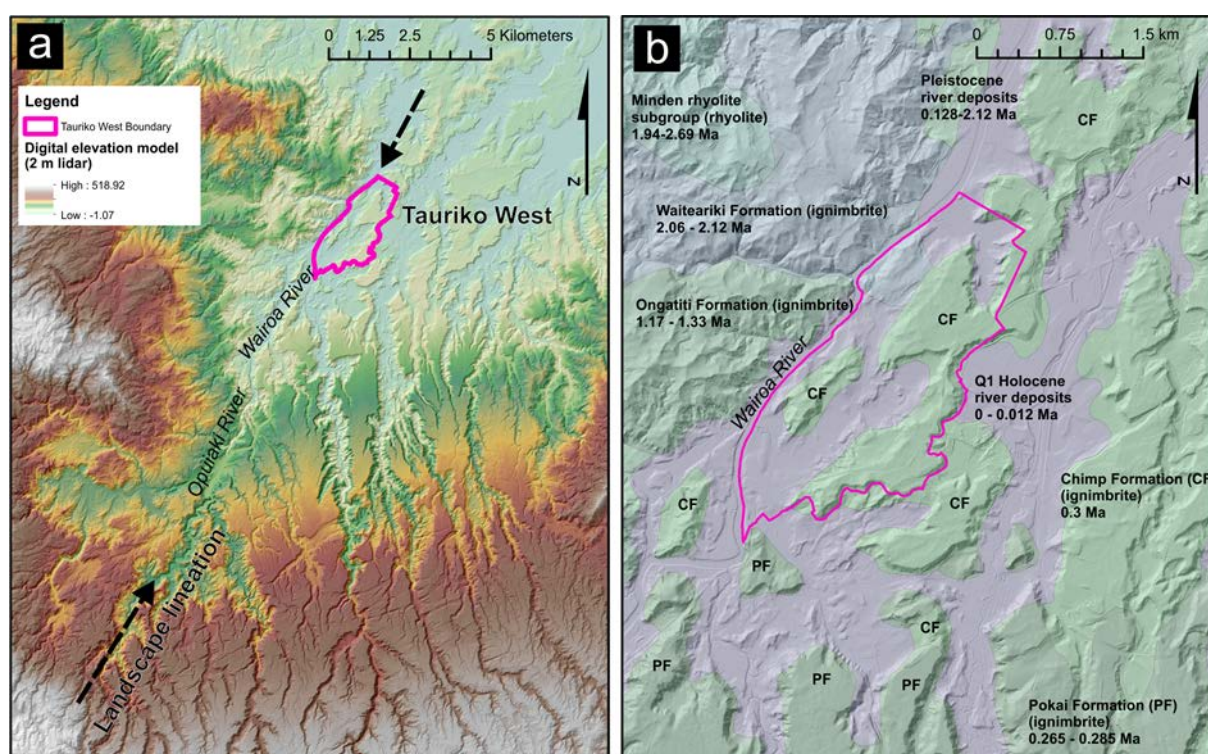
Figure 2.1 (a) A digital elevation and hillshade LiDAR DEM of the topography of the region surrounding the Tauriko West area. The black arrows point out the large-scale landscape lineation that may represent a fault line. (b) The geology and landform ages of the Tauriko West area, from Leonard et al. (2010).
