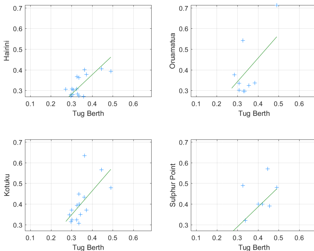
Figure 8-3: Comparison between large skew surges measured at Tug Berth with other gauges. Only surges in the top 3% are compared, except at Sulphur Point where all surges associated with matching annual maxima from Table C-1 are plotted (some outside the axis margins). Linear fits through 0,0 are also plotted.
