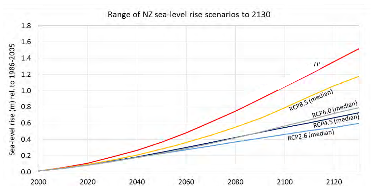
Figure 6-1: Range of sea-level rise scenarios to year 2130. Global average projections have been adjusted for New Zealand by adding up to 0.05 m to cover the slightly-higher expected SLR in the SW Pacific centred in NZ (Ackerley et al. 2013).
