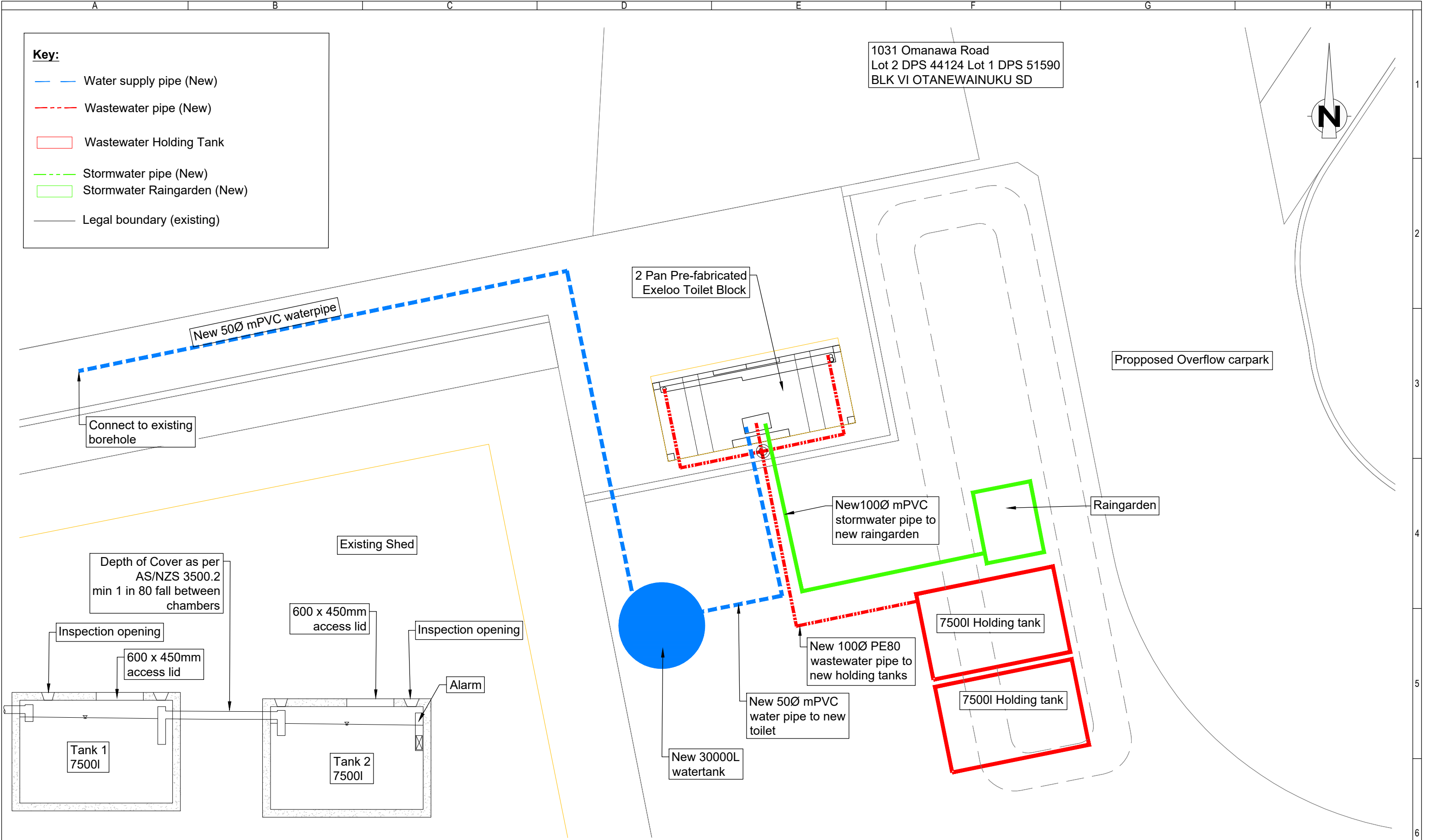
3 WATER LAYOUT Scale 1:100 on A3
