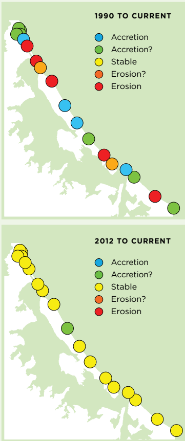
Figure 2: Overall change in beach shape at monitoring sites in Tauranga Moana between 1990 and 2017, and between 2012 and 2017.
