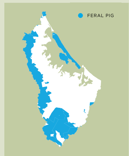
Figure 1: Distribution of some common mammalian pests in Tauranga Moana 30 .
