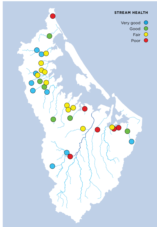
Figure 1: Grades (MCI scores) for the stream health indicator at sites around Tauranga Moana.
