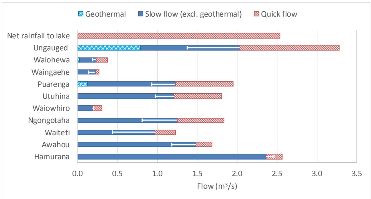
Figure 3.1: Inflow to Lake Rotorua from sub-catchments (2007-2014) indicating component of the total flow as quick flow, slow flow and any geothermal component of slow flow. Negative error bars assume a drainage factor of 0.5 weighted by relative groundwater catchment area (see D2 in Table 3.4). The range highlights the uncertainty around apportioning slow flow and quick flow in the ungauged catchments.
