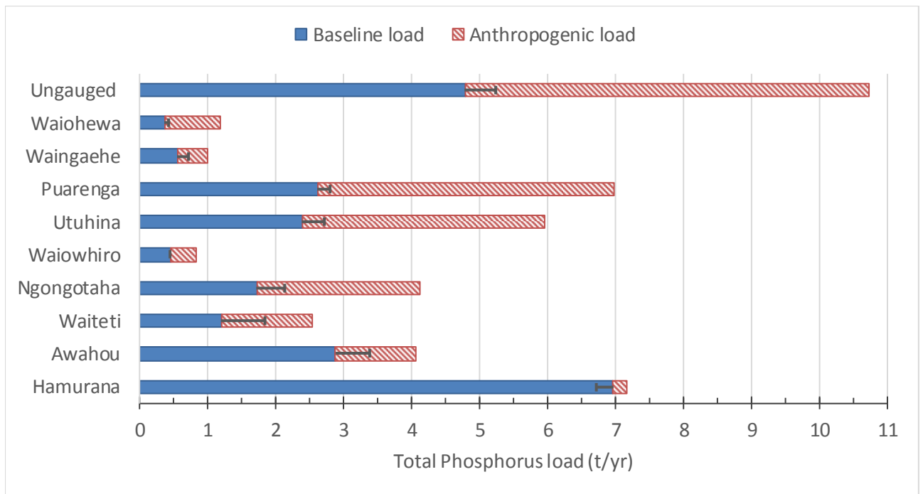
Figure 3.3: Total phosphorus load to Lake Rotorua (2007-2014) with the baseline and anthropogenic contributions indicated for drainage factor D2 and accounting for geothermal inputs. Error bars show scenario D1.
