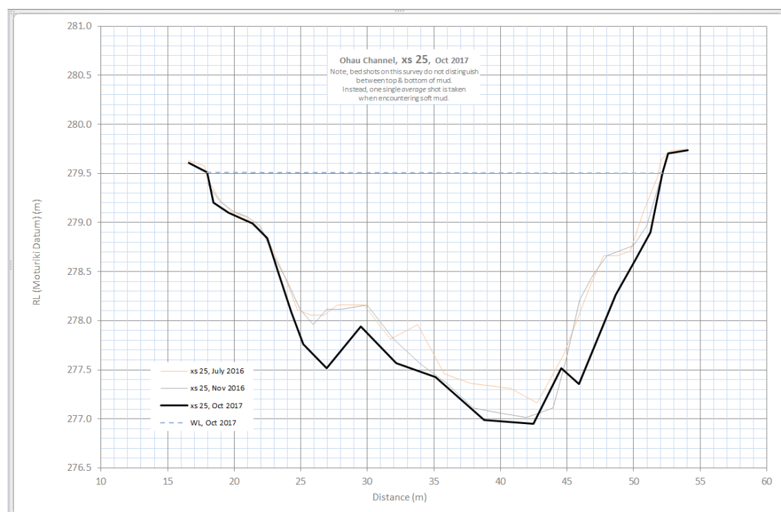
Figure 19 Cross section number 25 located above State Highway 33 – July 2016 to October 2017.
